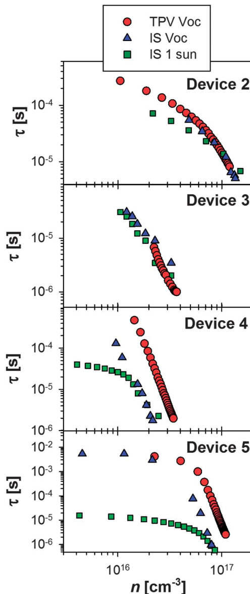
Fig. 5 Charge carrier lifetimes of representative devices based on either P3HT:PC _{60} BM or PTB7 at different carrier densities. TPV and IS measurements were performed under open circuit conditions and different illumination ( V_{oc} ) or under constant illumination.
